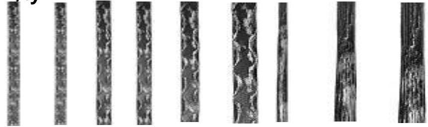
32.001 □ 12 H 3000 32.002 □ 12 H 6000 32.003 □ 14 H 3000 32.004 □ 14 H 6000 32.005 □ 16 H 3000 32.006 □ 20 H 3000 32.100 ∅10-∅12 H 1100 32.101 ∅ 12 - ∅16 H 1100 32.12 ∅ 12 - ∅20 H 1100
